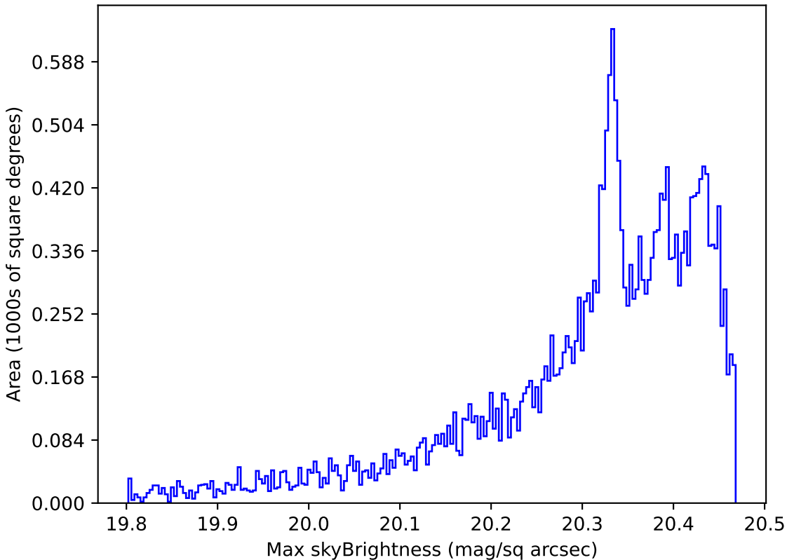
all_long_v3.4_10yrs All sky i band: Max skyBrightness
