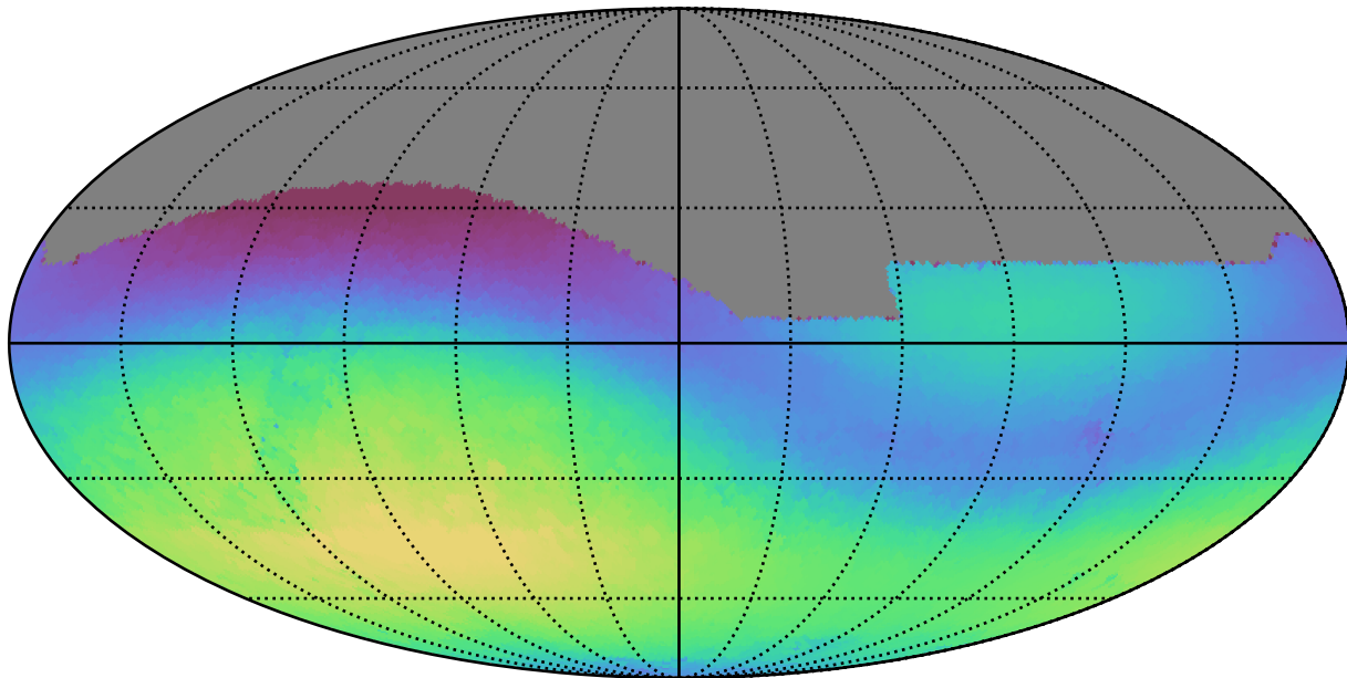
all_long_v3.4_10yrs All sky g band: Max skyBrightness
