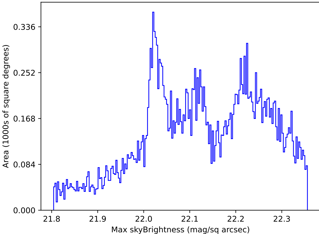
all_long_v3.4_10yrs All sky g band: Max skyBrightness
