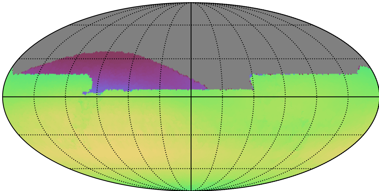
all_long_v3.4_10yrs All sky all bands: Max skyBrightness
