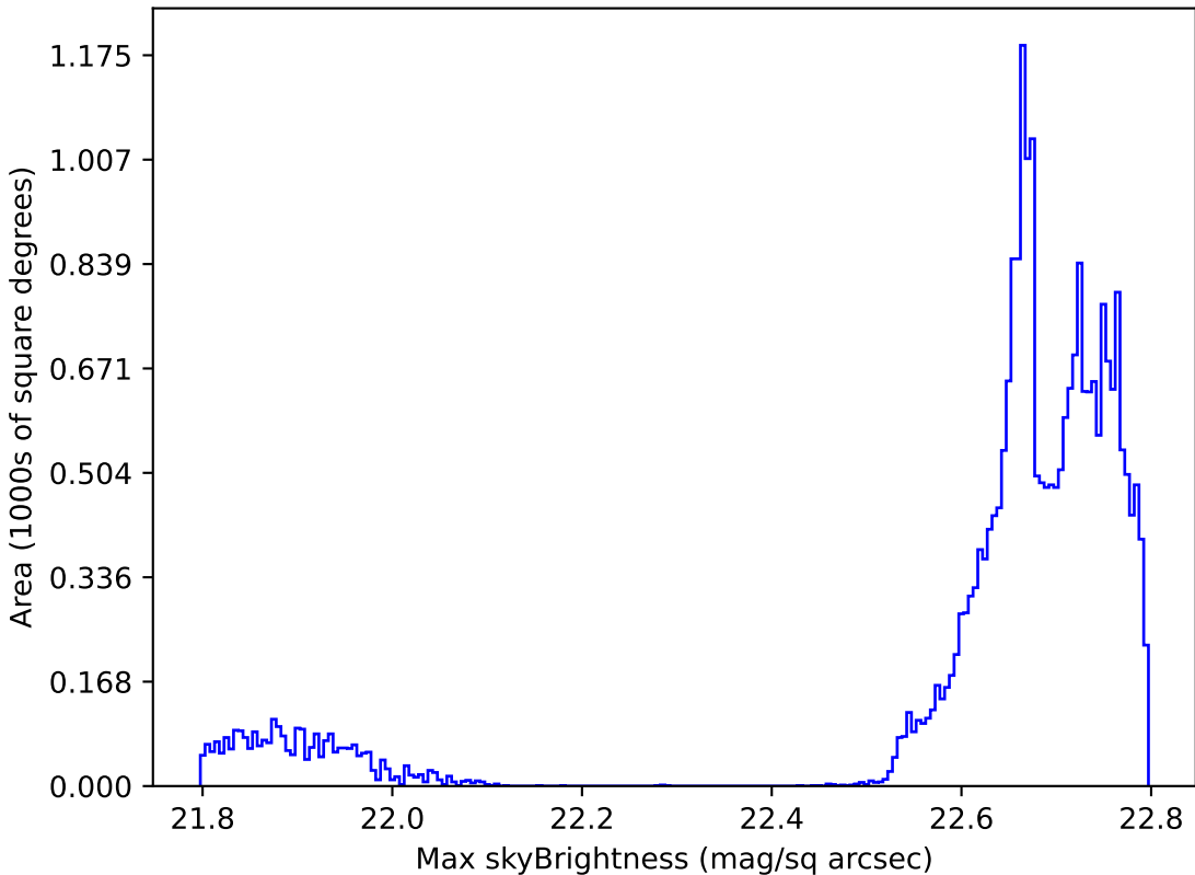
all_long_v3.4_10yrs All sky all bands: Max skyBrightness
