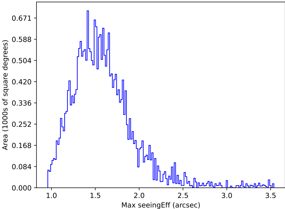
all_long_v3.4_10yrs Yr 1 z band: Max seeingEff
