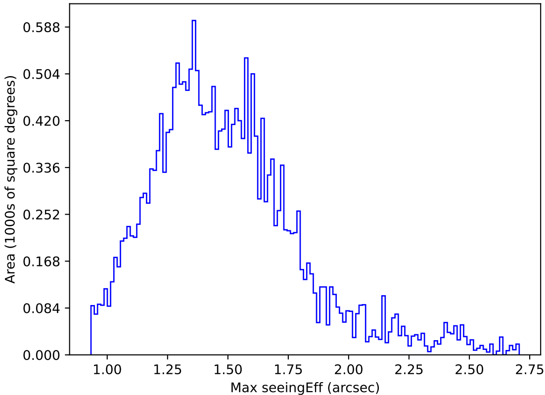
all_long_v3.4_10yrs Yr 1 y band: Max seeingEff
