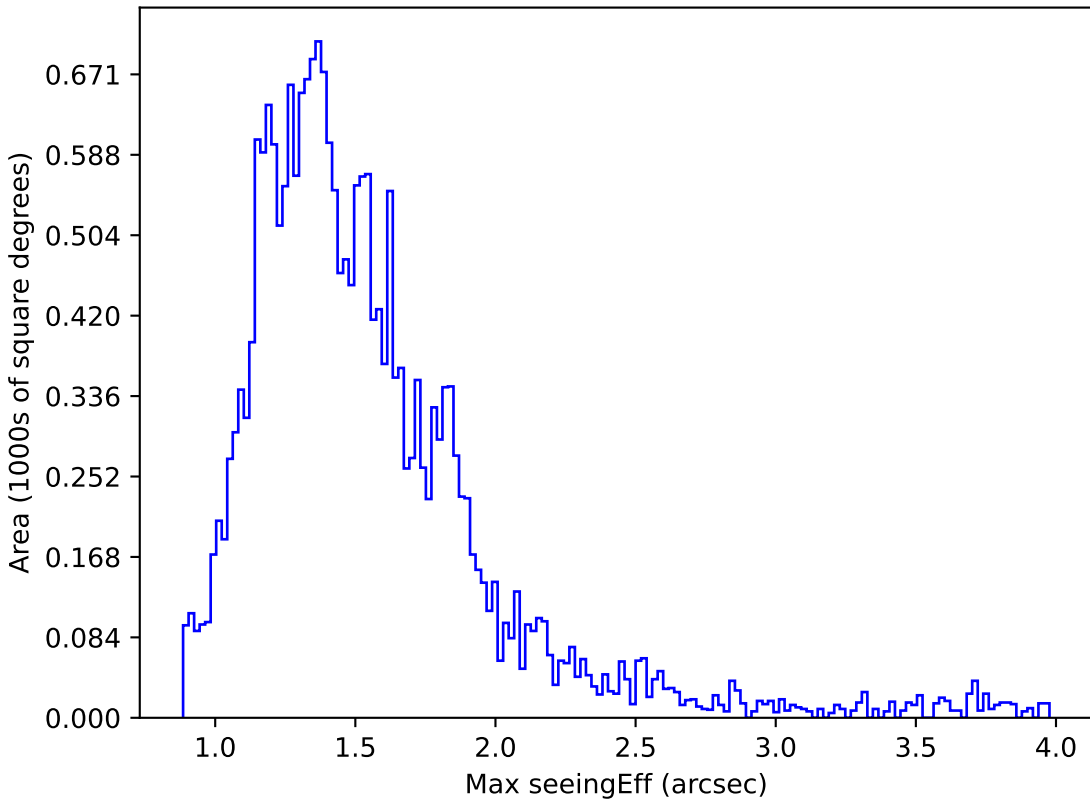
all_long_v3.4_10yrs Yr 1 u band: Max seeingEff
