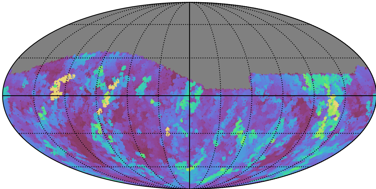
all_long_v3.4_10yrs Yr 1 r band: Max seeingEff
