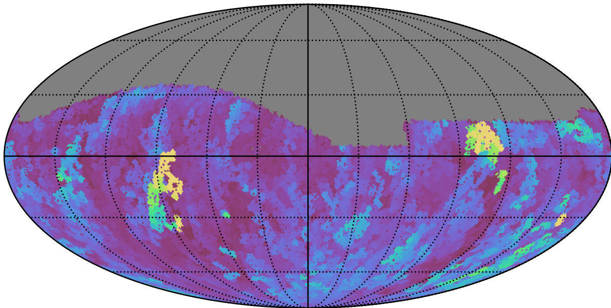
all_long_v3.4_10yrs Yr 1 g band: Max seeingEff
