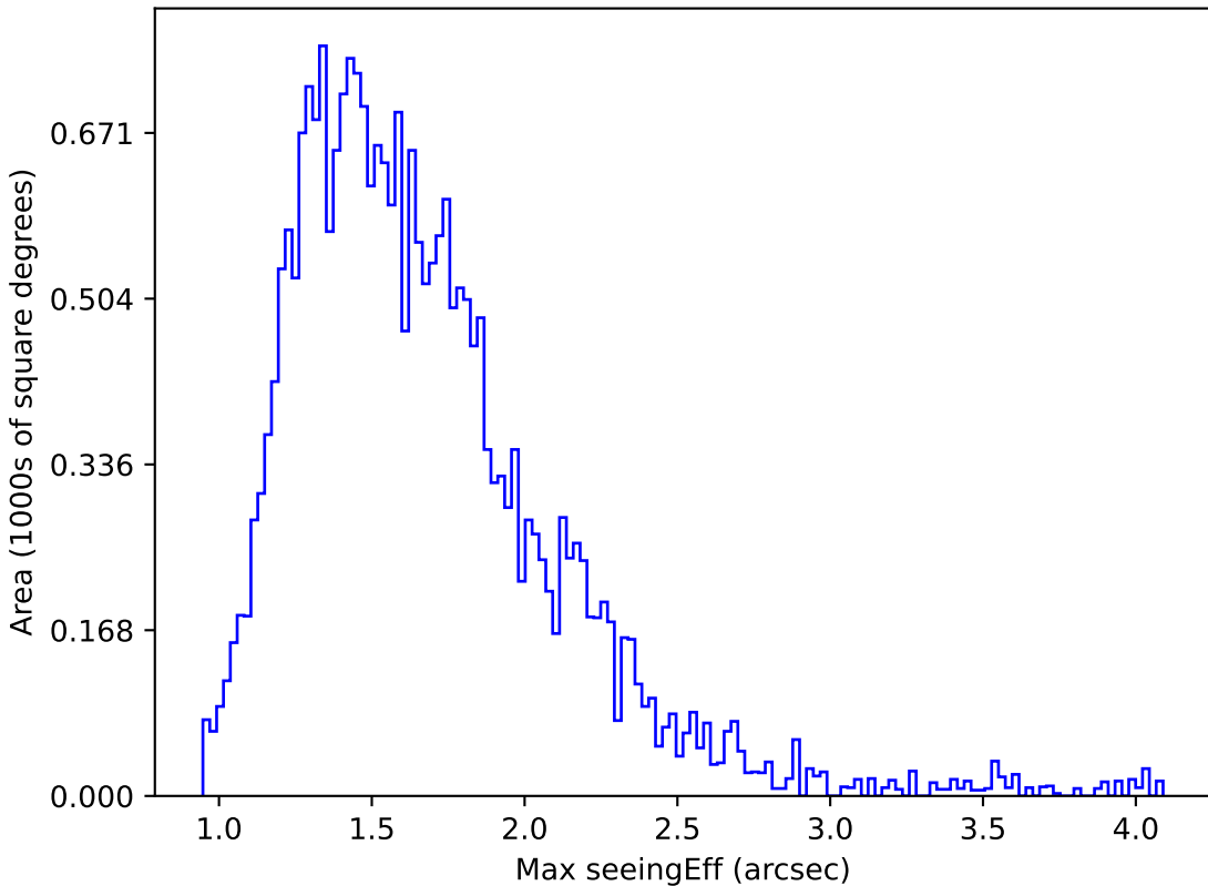
all_long_v3.4_10yrs Yr 1 g band: Max seeingEff
