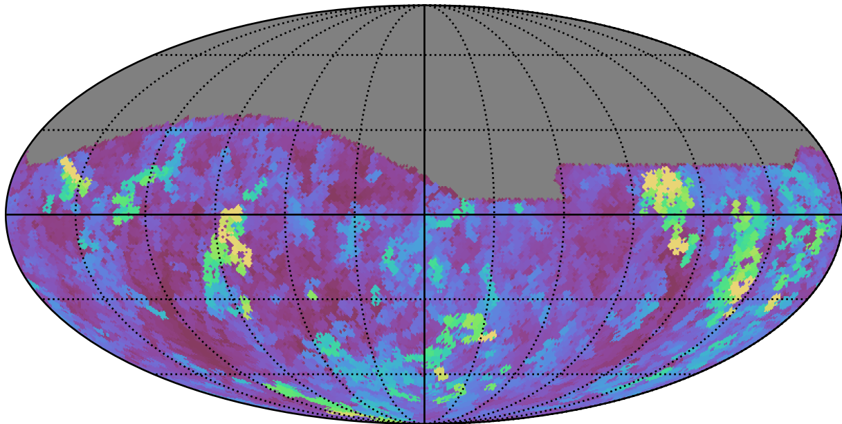
all_long_v3.4_10yrs Yr 1 all bands: Max seeingEff
