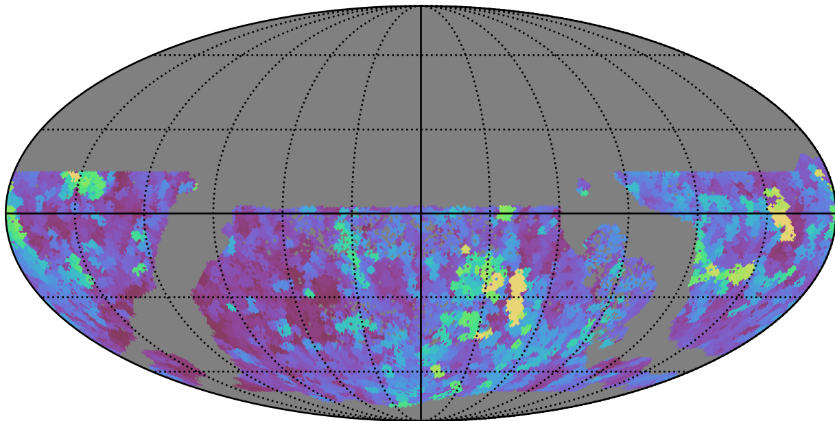
all_long_v3.4_10yrs WFD z band: Max seeingEff
