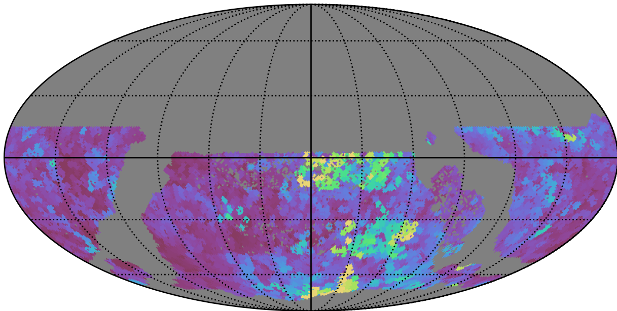
all_long_v3.4_10yrs WFD y band: Max seeingEff
