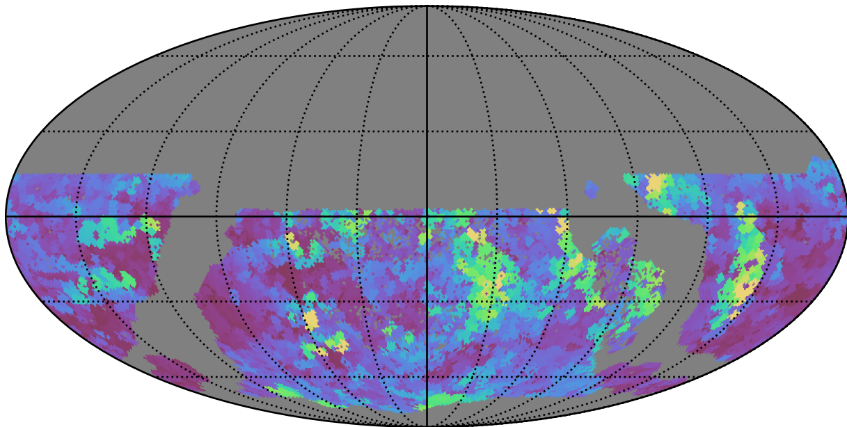
all_long_v3.4_10yrs WFD u band: Max seeingEff
