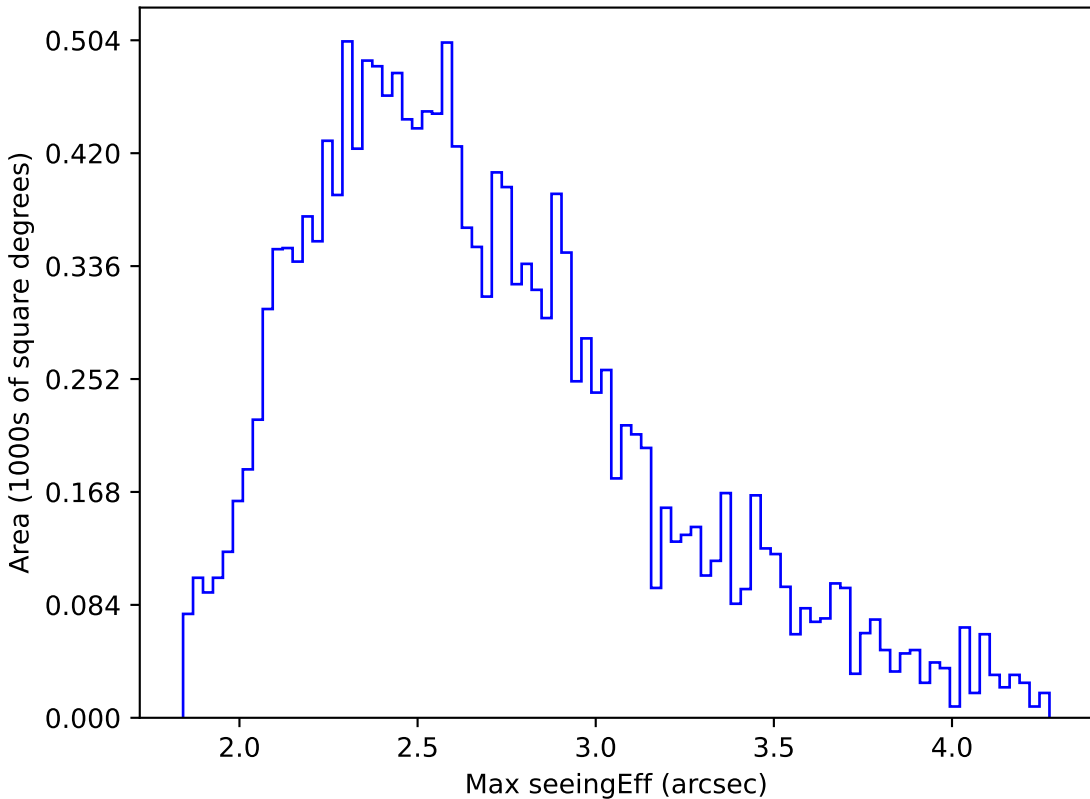
all_long_v3.4_10yrs WFD r band: Max seeingEff
