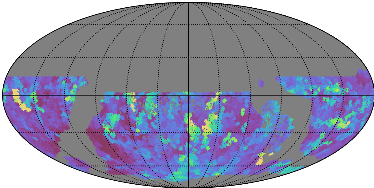
all_long_v3.4_10yrs WFD i band: Max seeingEff
