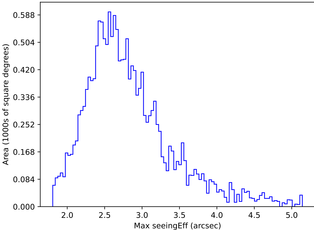
all_long_v3.4_10yrs WFD i band: Max seeingEff
