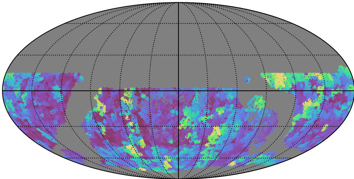
all_long_v3.4_10yrs WFD g band: Max seeingEff
