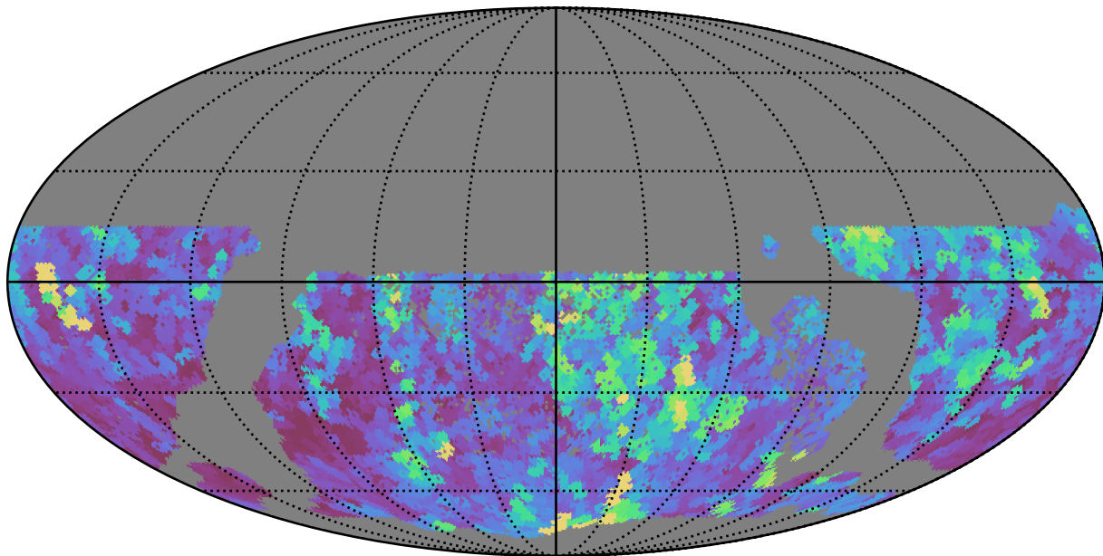
all_long_v3.4_10yrs WFD all bands: Max seeingEff
