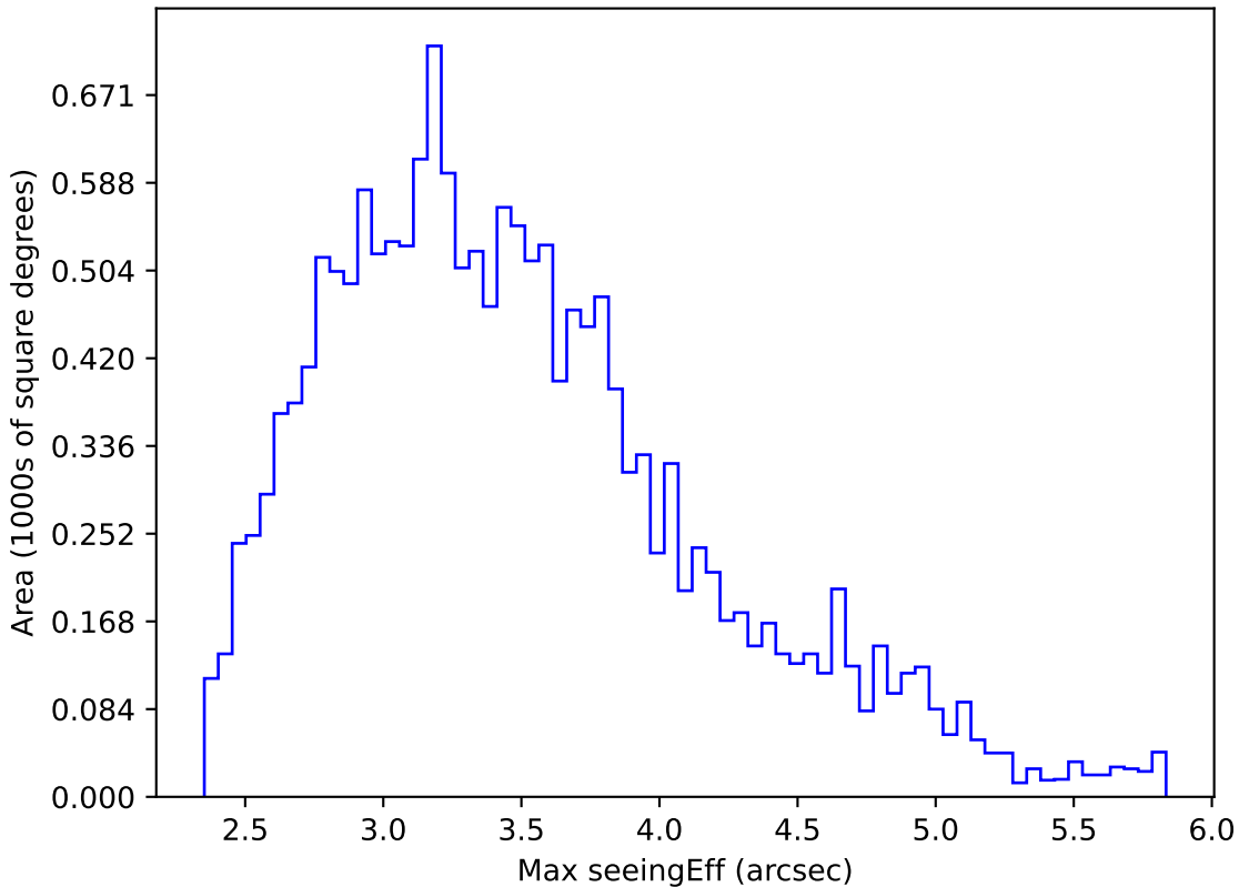
all_long_v3.4_10yrs WFD all bands: Max seeingEff
