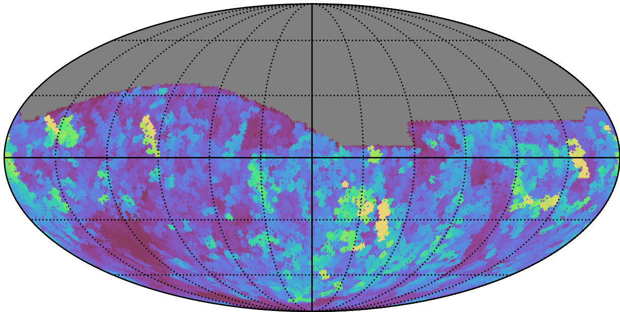
all_long_v3.4_10yrs All sky z band: Max seeingEff
