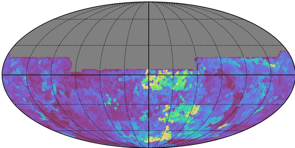
all_long_v3.4_10yrs All sky y band: Max seeingEff
