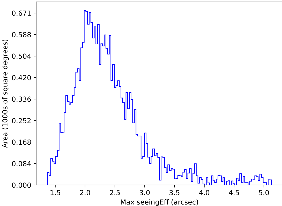
all_long_v3.4_10yrs All sky y band: Max seeingEff
