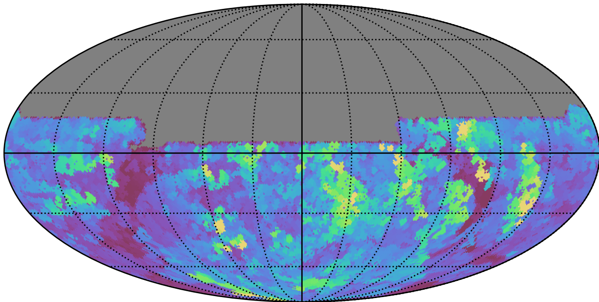
all_long_v3.4_10yrs All sky u band: Max seeingEff
