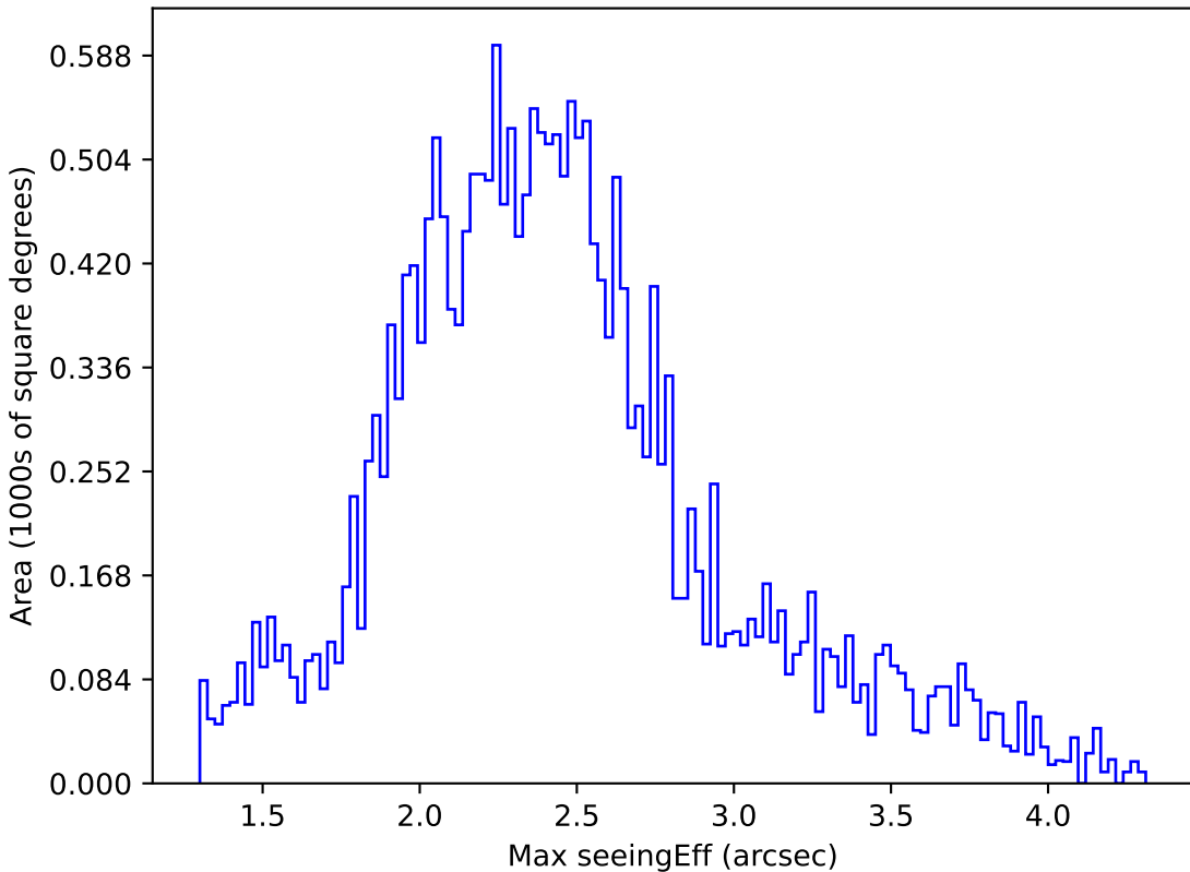
all_long_v3.4_10yrs All sky u band: Max seeingEff
