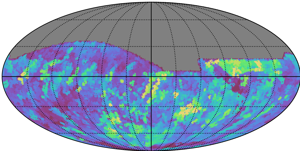
all_long_v3.4_10yrs All sky r band: Max seeingEff
