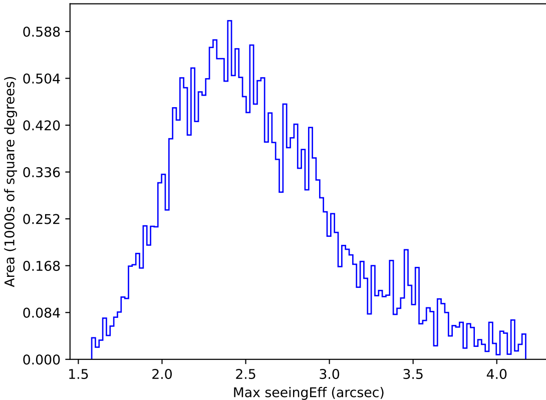
all_long_v3.4_10yrs All sky r band: Max seeingEff
