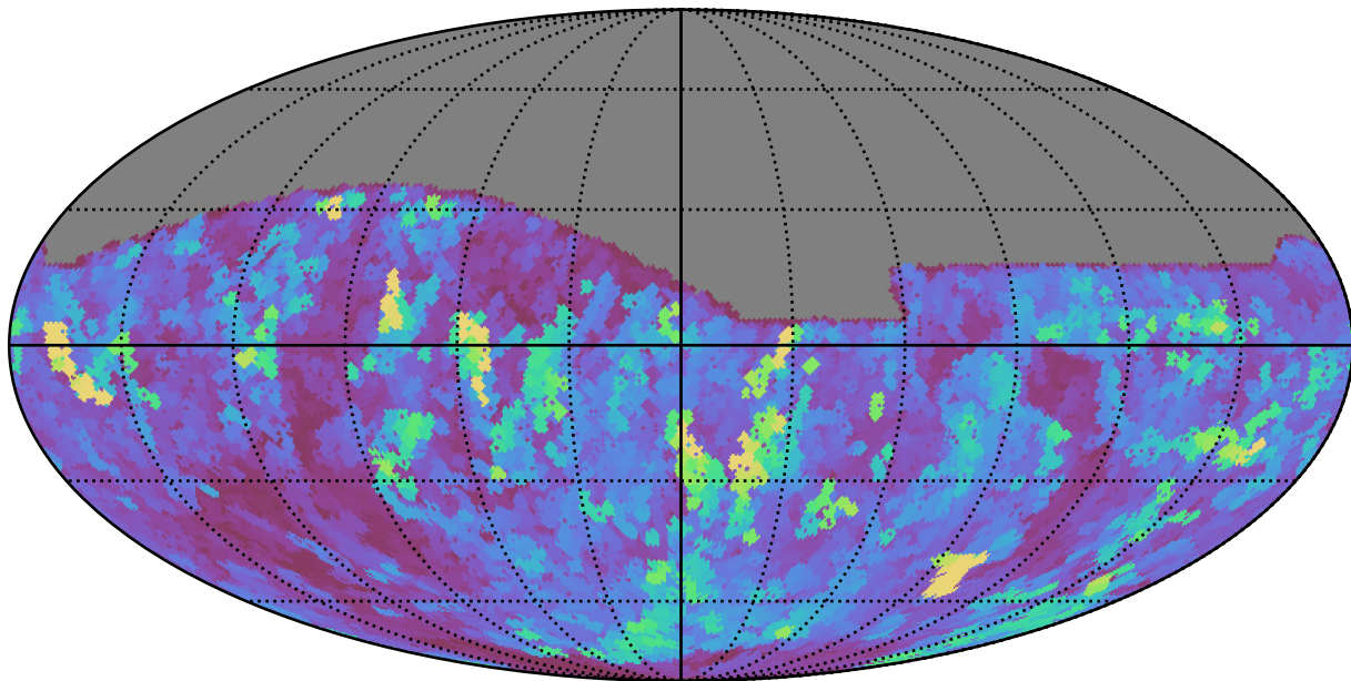
all_long_v3.4_10yrs All sky i band: Max seeingEff
