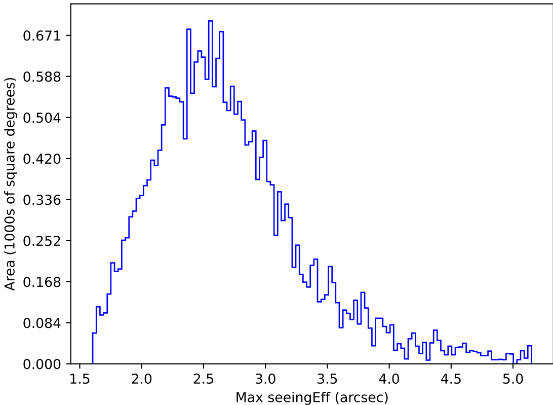
all_long_v3.4_10yrs All sky i band: Max seeingEff
