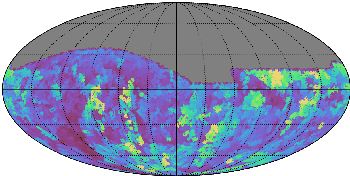
all_long_v3.4_10yrs All sky g band: Max seeingEff
