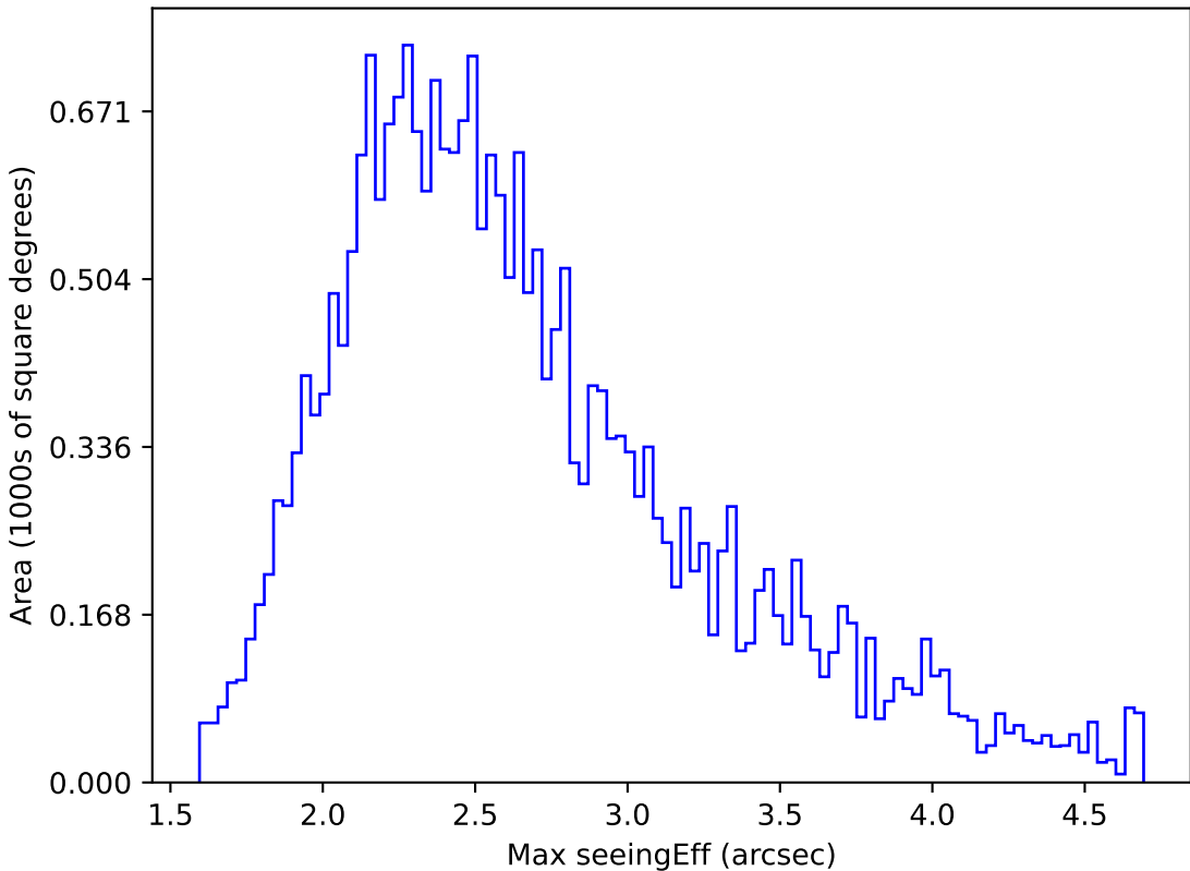
all_long_v3.4_10yrs All sky g band: Max seeingEff
