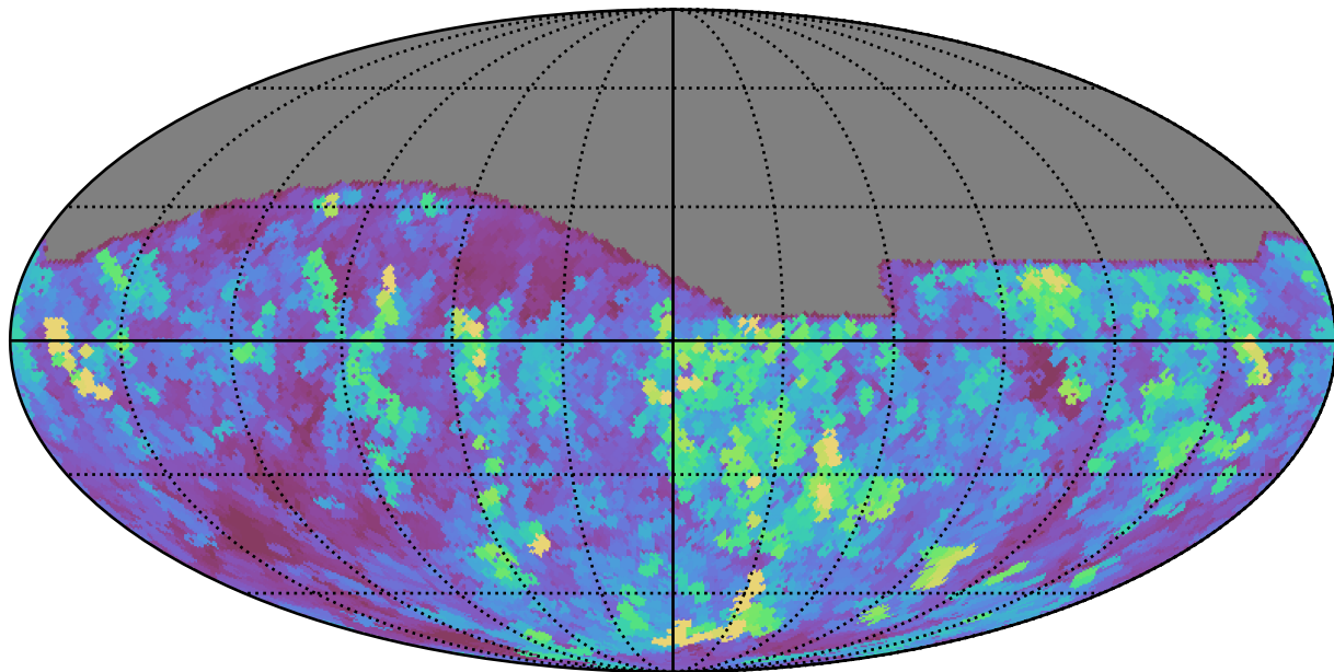
all_long_v3.4_10yrs All sky all bands: Max seeingEff
