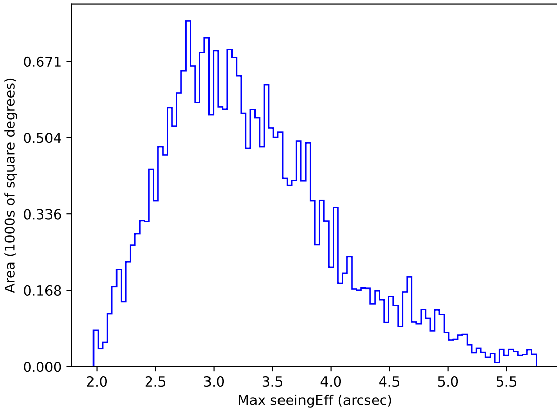
all_long_v3.4_10yrs All sky all bands: Max seeingEff
