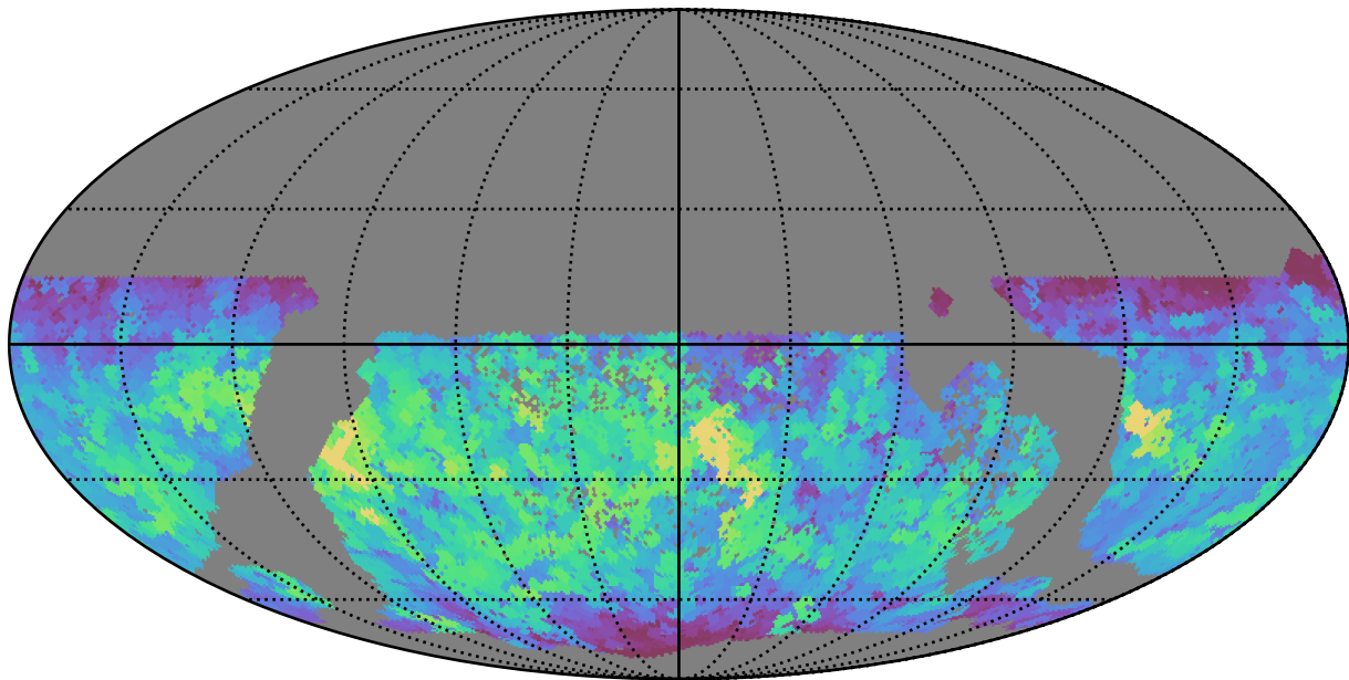
all_long_v3.4_10yrs WFD z band: Max saturation_mag
