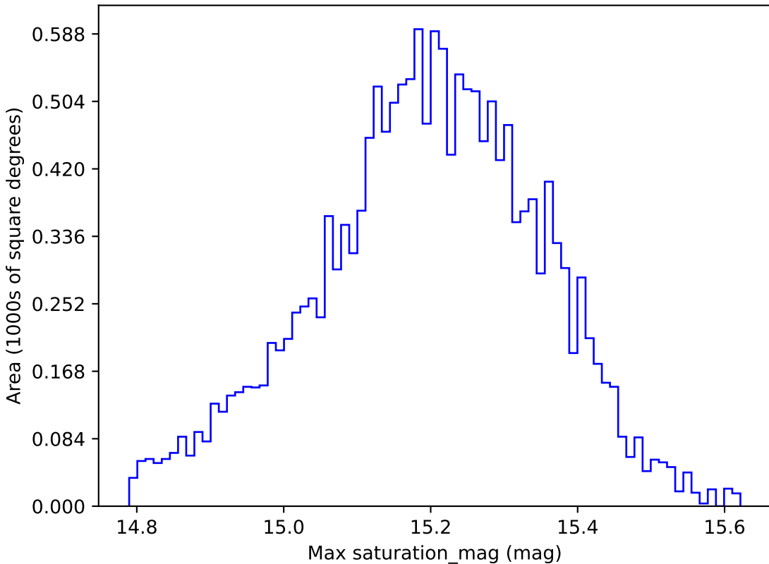
all_long_v3.4_10yrs WFD z band: Max saturation_mag
