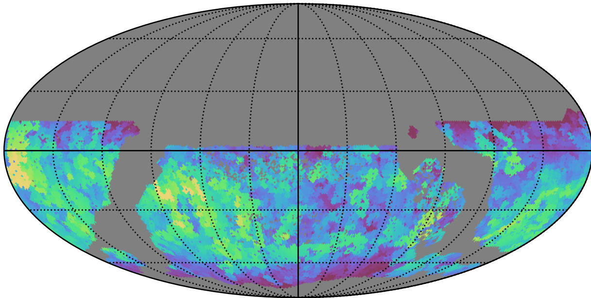
all_long_v3.4_10yrs WFD u band: Max saturation_mag
