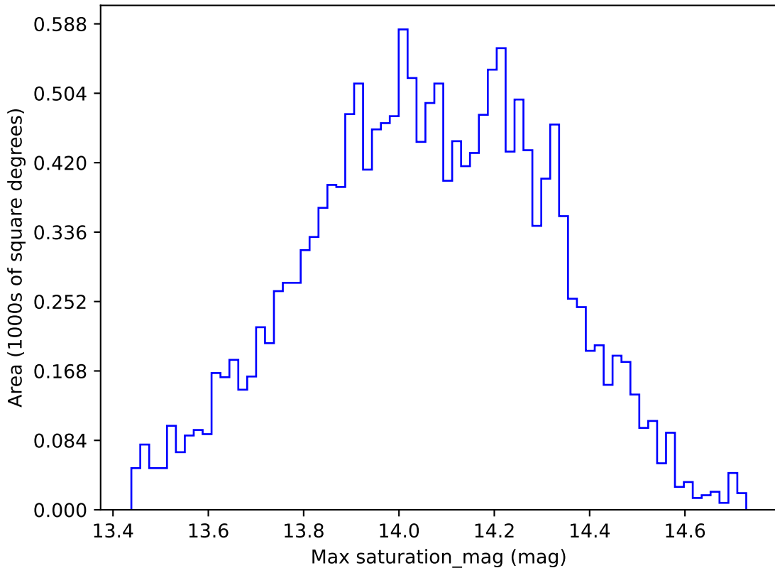
all_long_v3.4_10yrs WFD u band: Max saturation_mag
