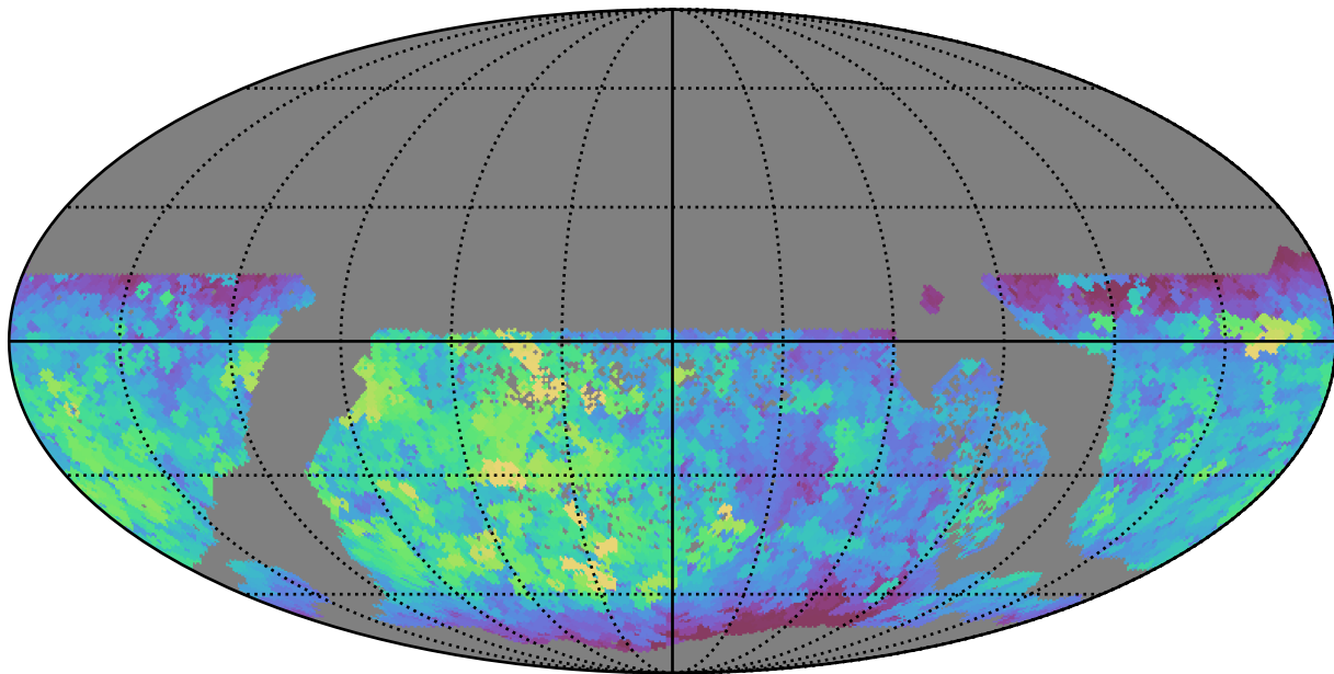
all_long_v3.4_10yrs WFD r band: Max saturation_mag
