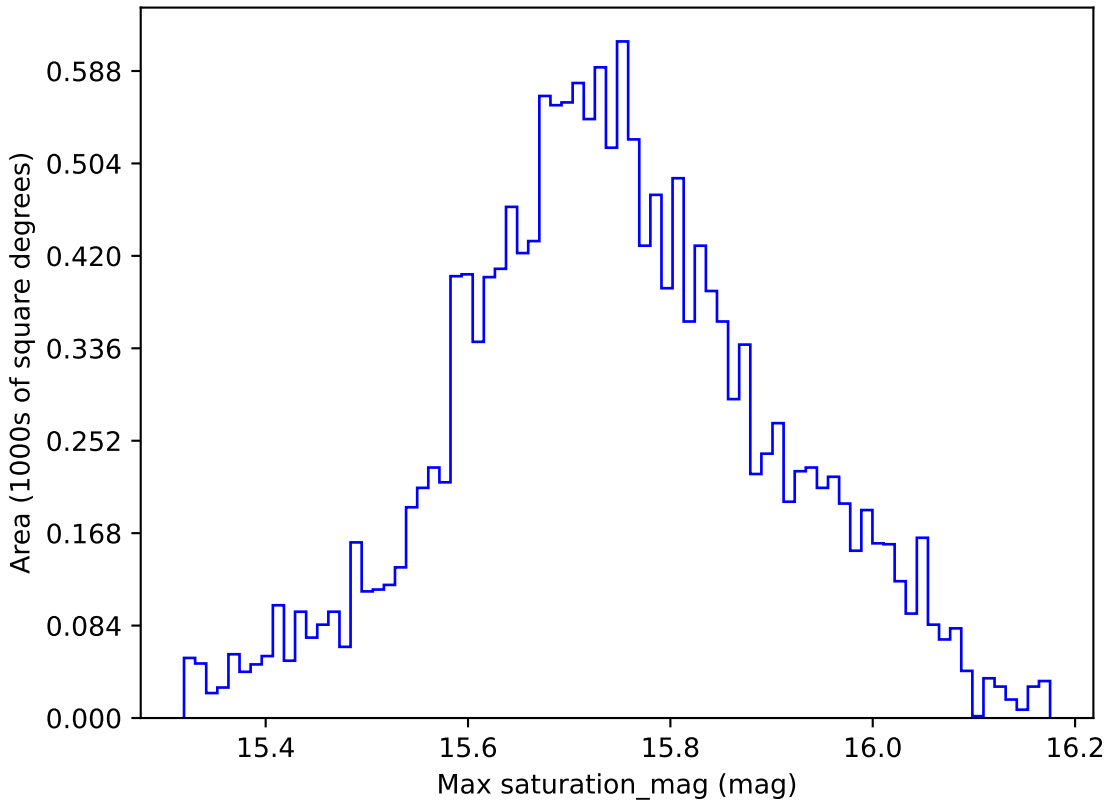
all_long_v3.4_10yrs WFD r band: Max saturation_mag
