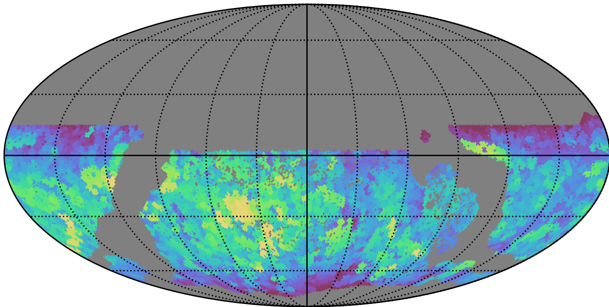
all_long_v3.4_10yrs WFD i band: Max saturation_mag
