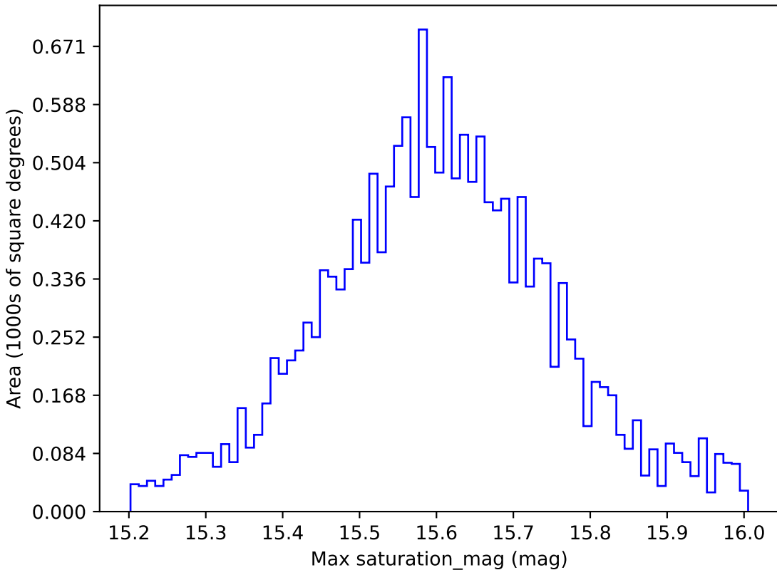
all_long_v3.4_10yrs WFD i band: Max saturation_mag
