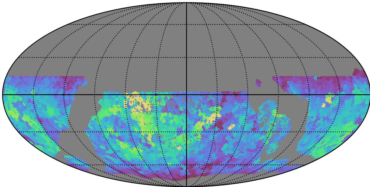
all_long_v3.4_10yrs WFD g band: Max saturation_mag
