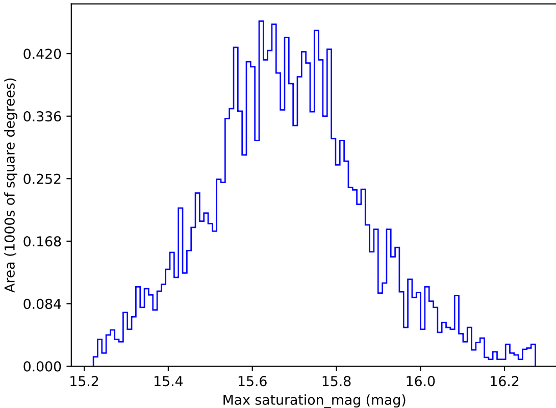
all_long_v3.4_10yrs WFD g band: Max saturation_mag
