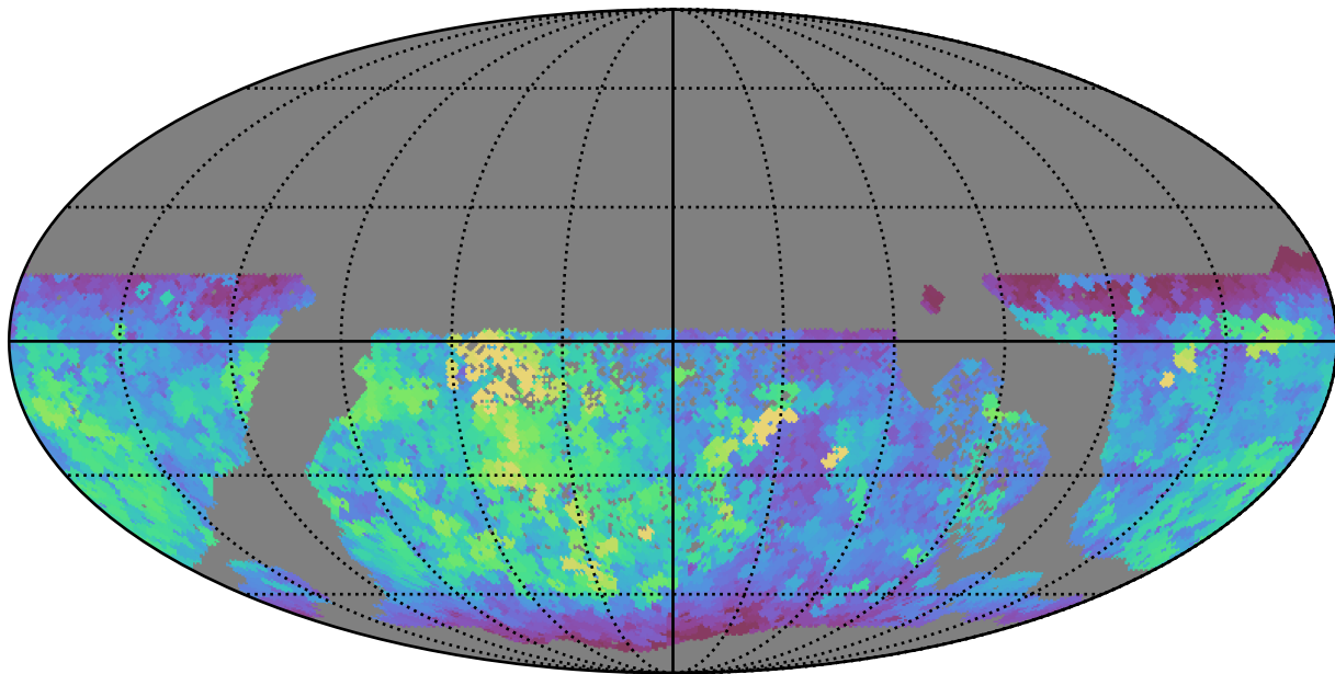
all_long_v3.4_10yrs WFD all bands: Max saturation_mag
