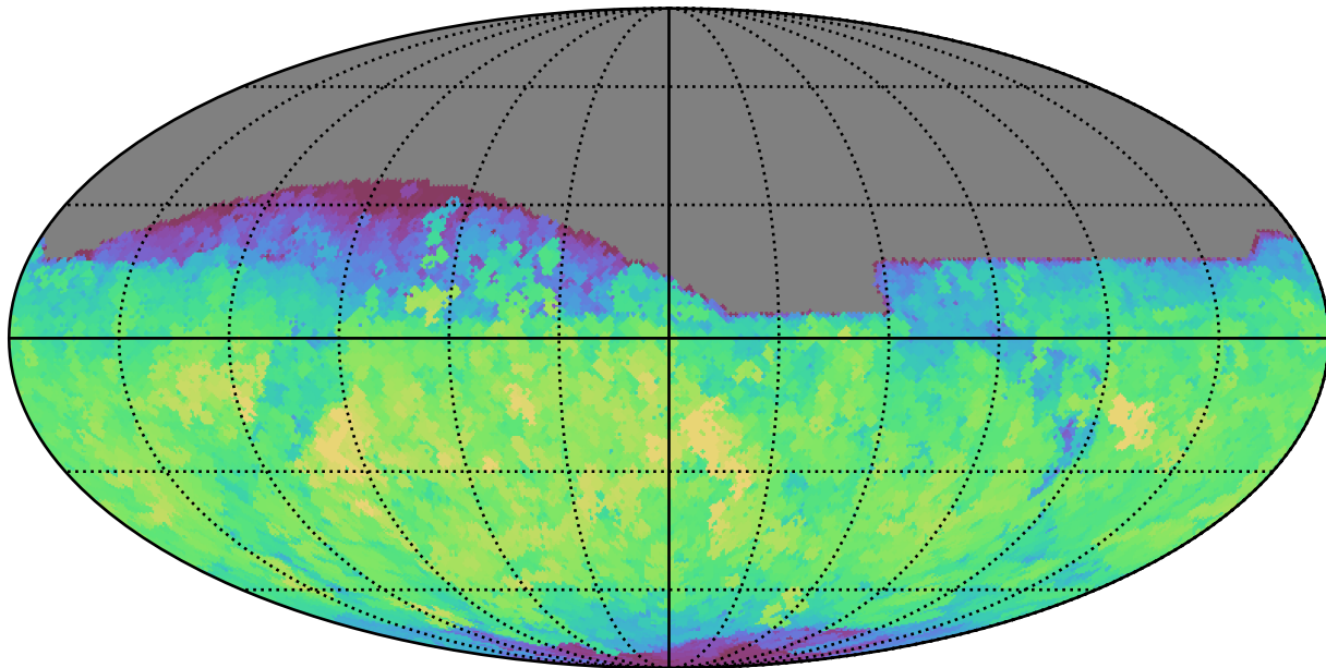
all_long_v3.4_10yrs All sky z band: Max saturation_mag
