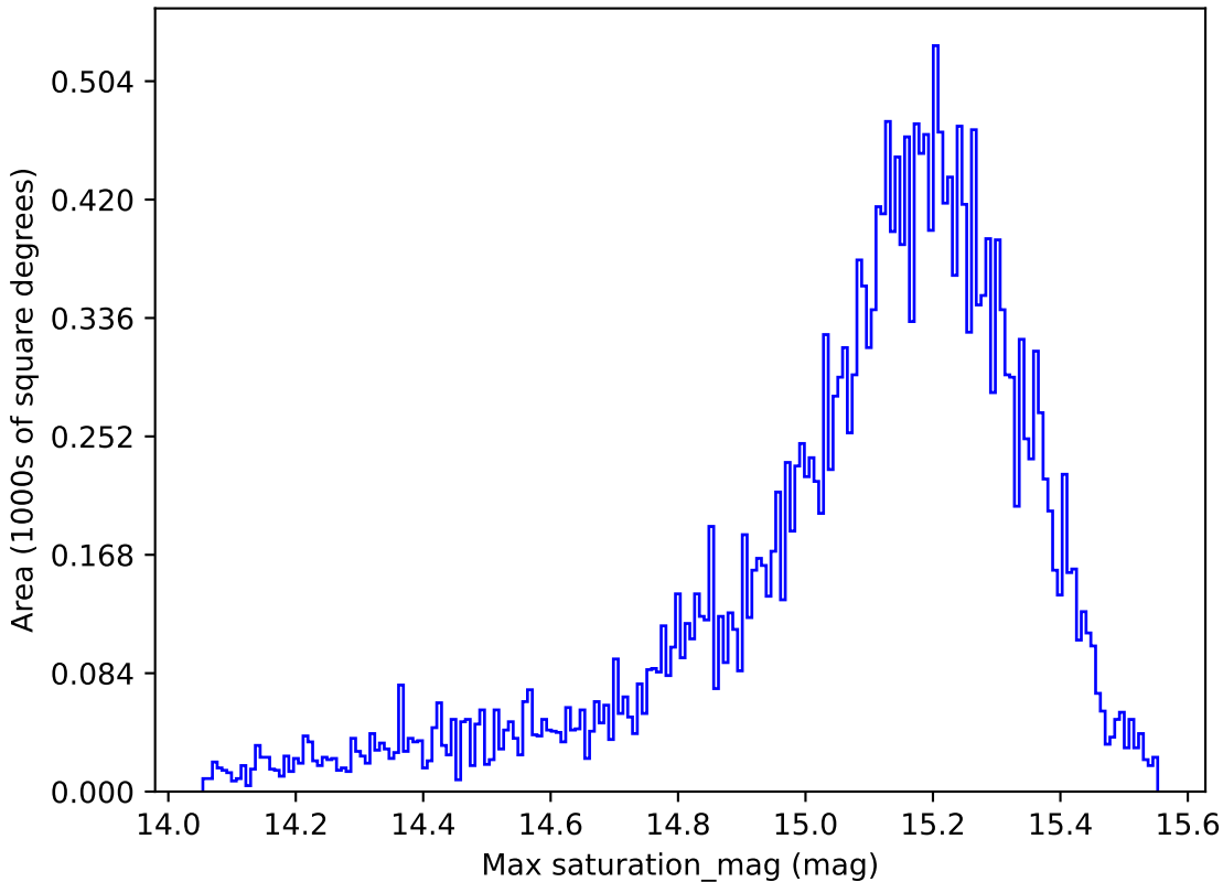
all_long_v3.4_10yrs All sky z band: Max saturation_mag
