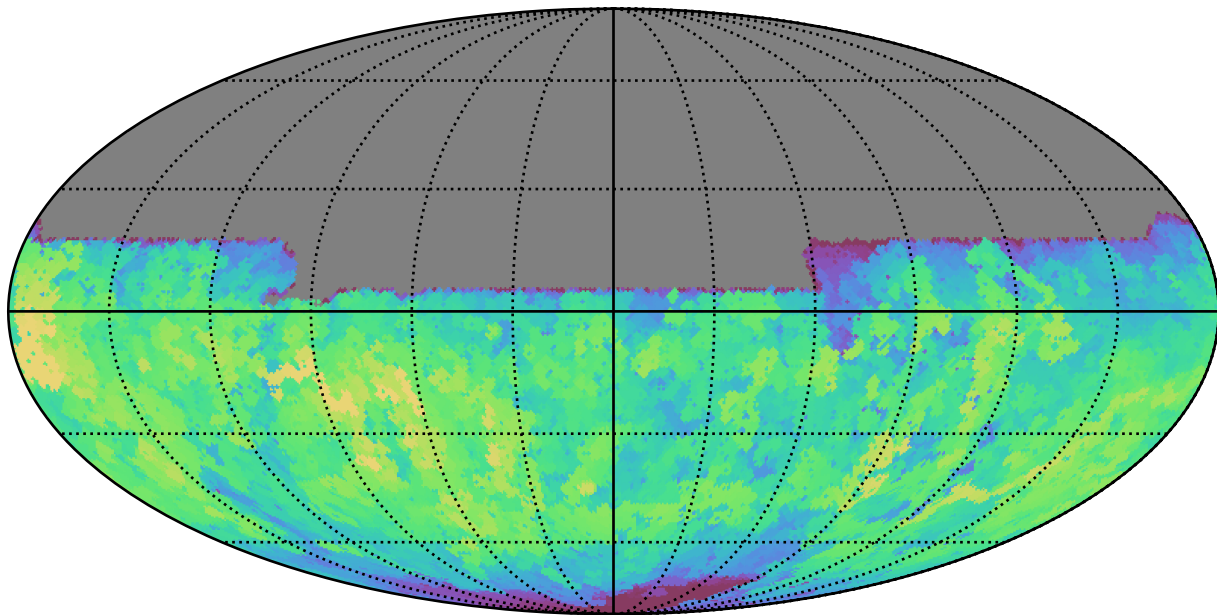
all_long_v3.4_10yrs All sky u band: Max saturation_mag
