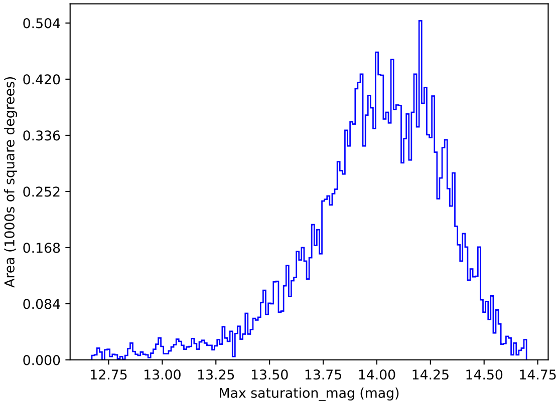
all_long_v3.4_10yrs All sky u band: Max saturation_mag
