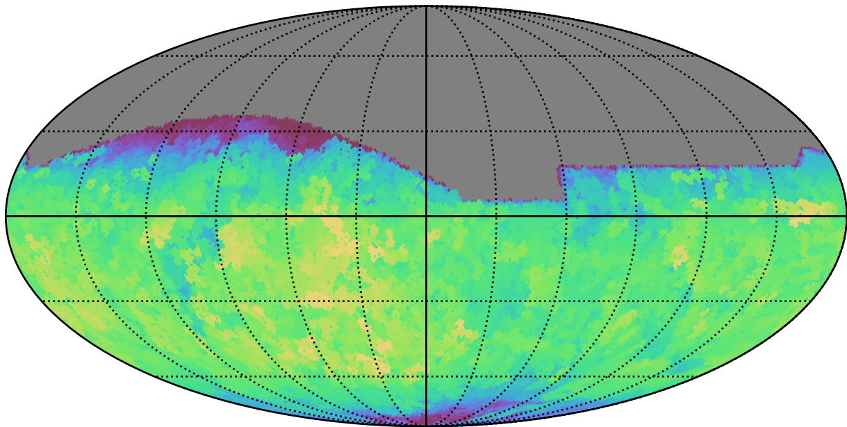
all_long_v3.4_10yrs All sky r band: Max saturation_mag
